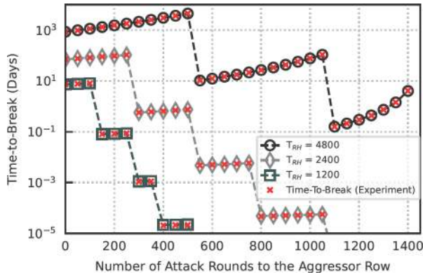
Fig. 6. Time-to-break RRS [51] with Juggernaut with varying attack rounds - both analytical and experimental results are shown. This analysis uses a swap rate of 6 for RRS. Juggernaut can break RRS in under 4 hours.
